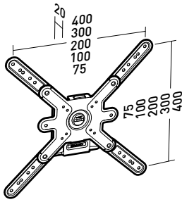
Mounting plate
