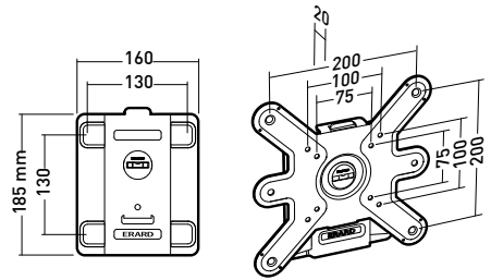
Wall mount
