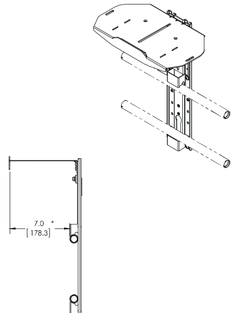
FUSION WALL ABOVE MOUNT SETUP
