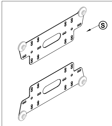
Supporto monitor Vesa 200 Vesa 200 Monitor sustain (x2)
