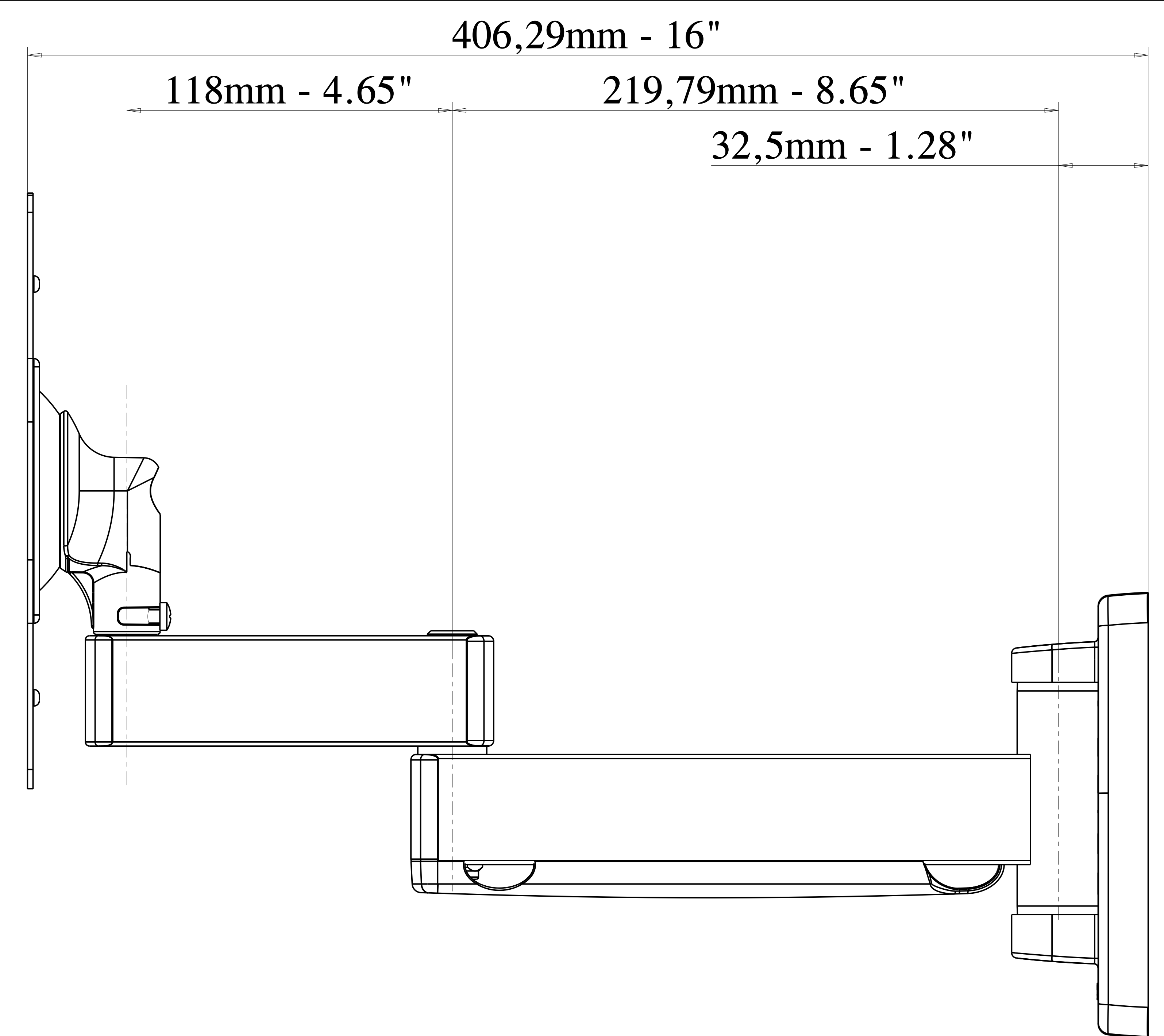
VISTA LATERALE - SIDE VIEW
