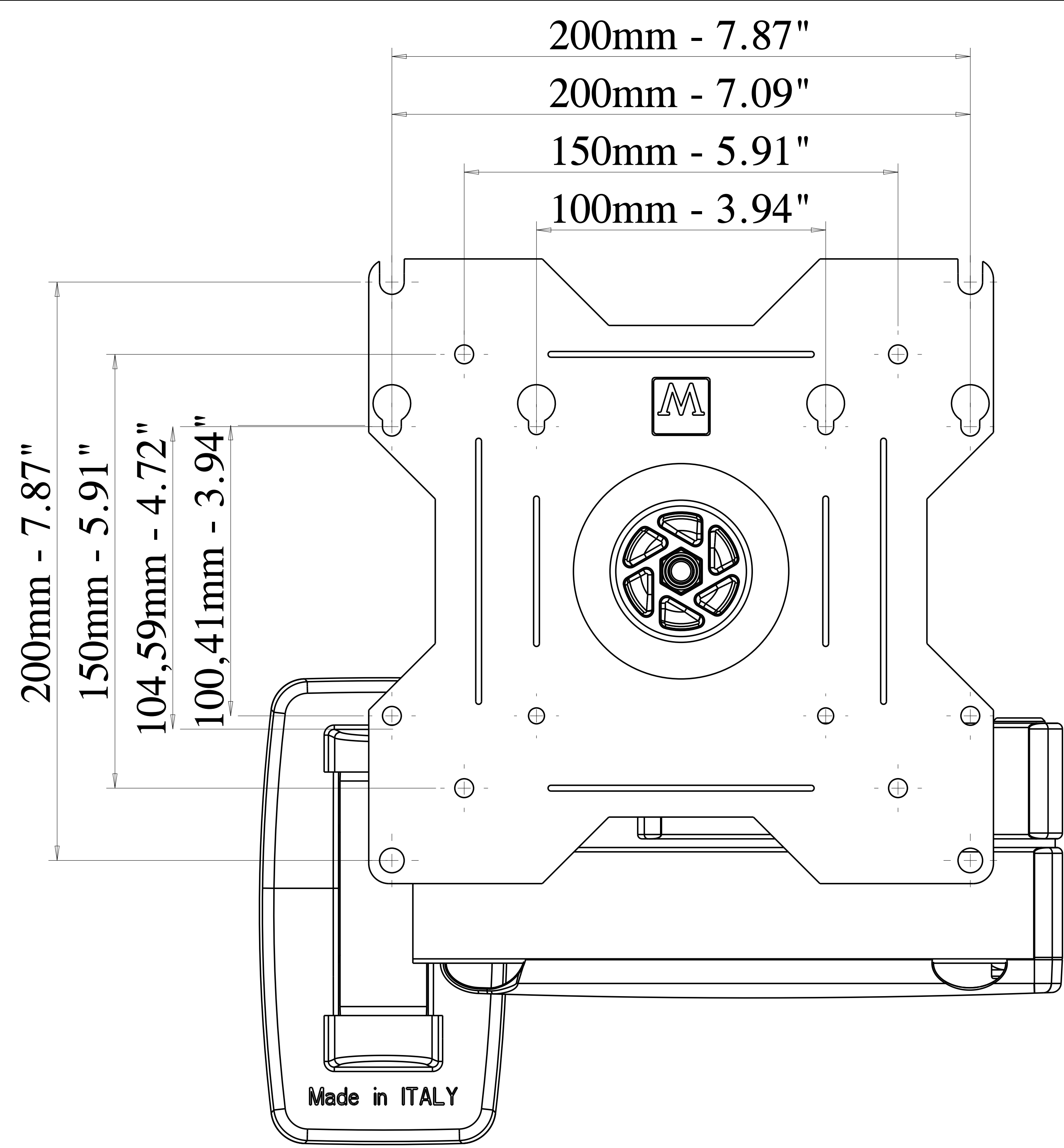
VISTA FRONTALE - FRONT VIEW
