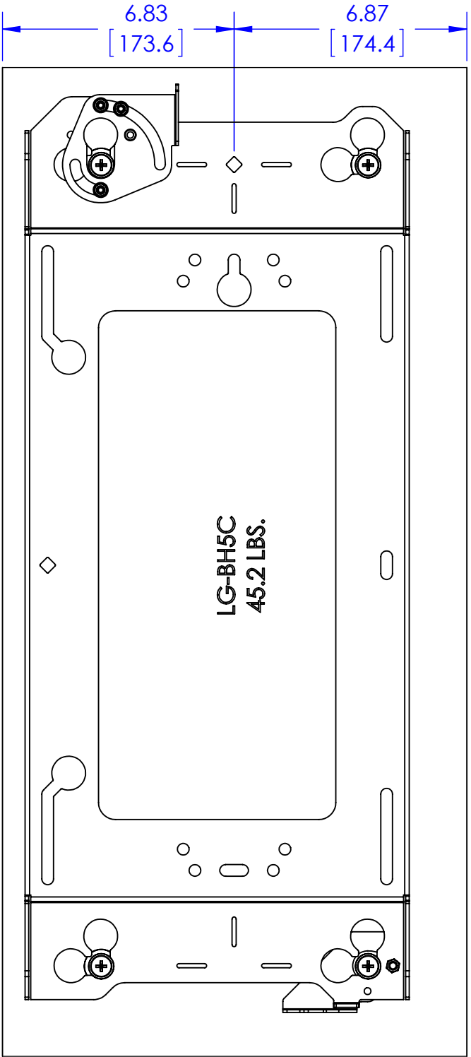
DETAIL C
