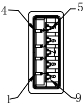
USB 3.0 A Male
