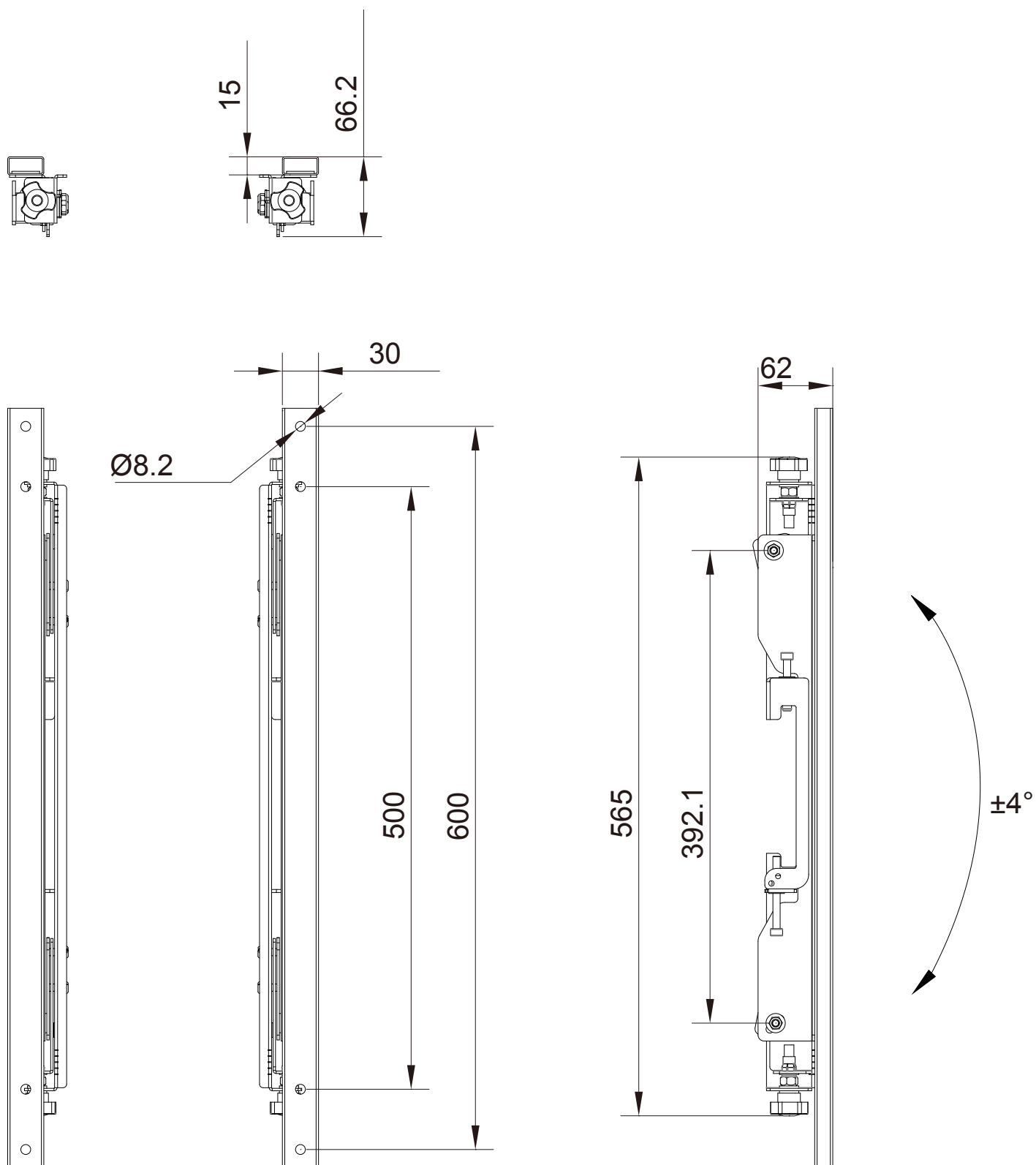
Technical measurements(mm)
